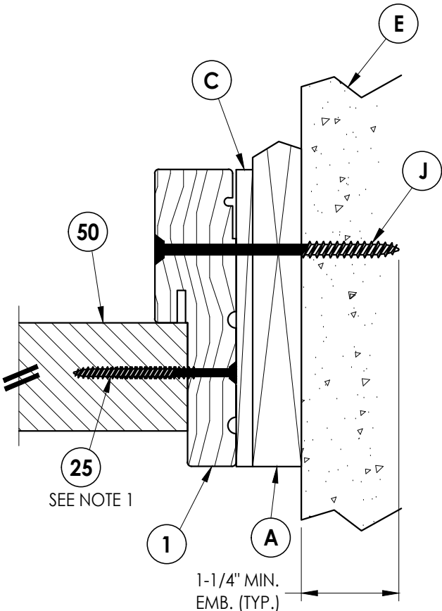
2 HORIZONTAL CROSS SECTION Shown w/ 1X sub-buck Outswing shown (Inswing similar)
